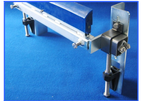
Figure 8. Tensioner devices CIAO PX and CIAO PX-R .
