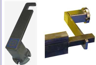
Figure 2: Tensioning device CRESA type RER (size 40). Figure 3: CRESA type RER (size 40) application.
