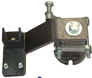
Figure 6. Tensioning devices CRESA type RERU (size 40).
