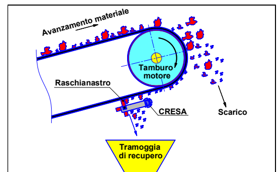
Drawing of a conveyor belt with belt scraper supports.
